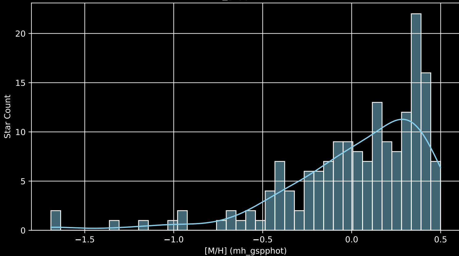
APOGEE DR17 Field: [SMC3 [M/H] (mh_gspphot) (n= 170)
