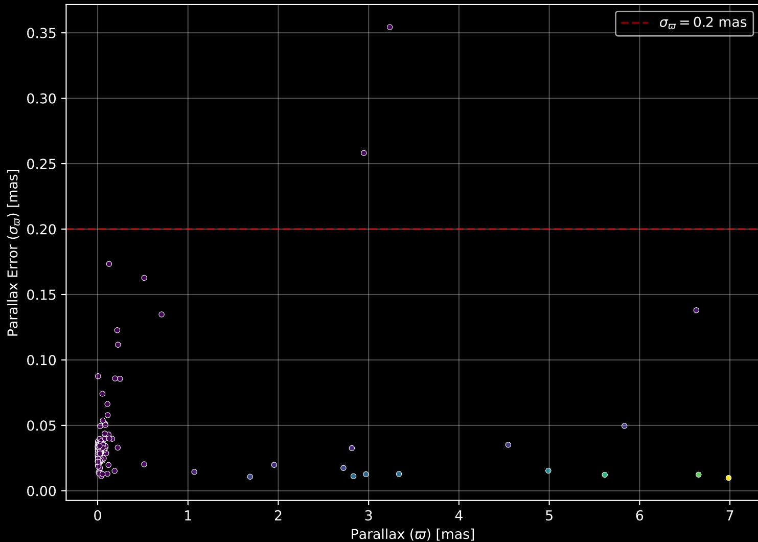
APOGEE DR17 Field: [SMC3] Parallax Quality (n= 180)
