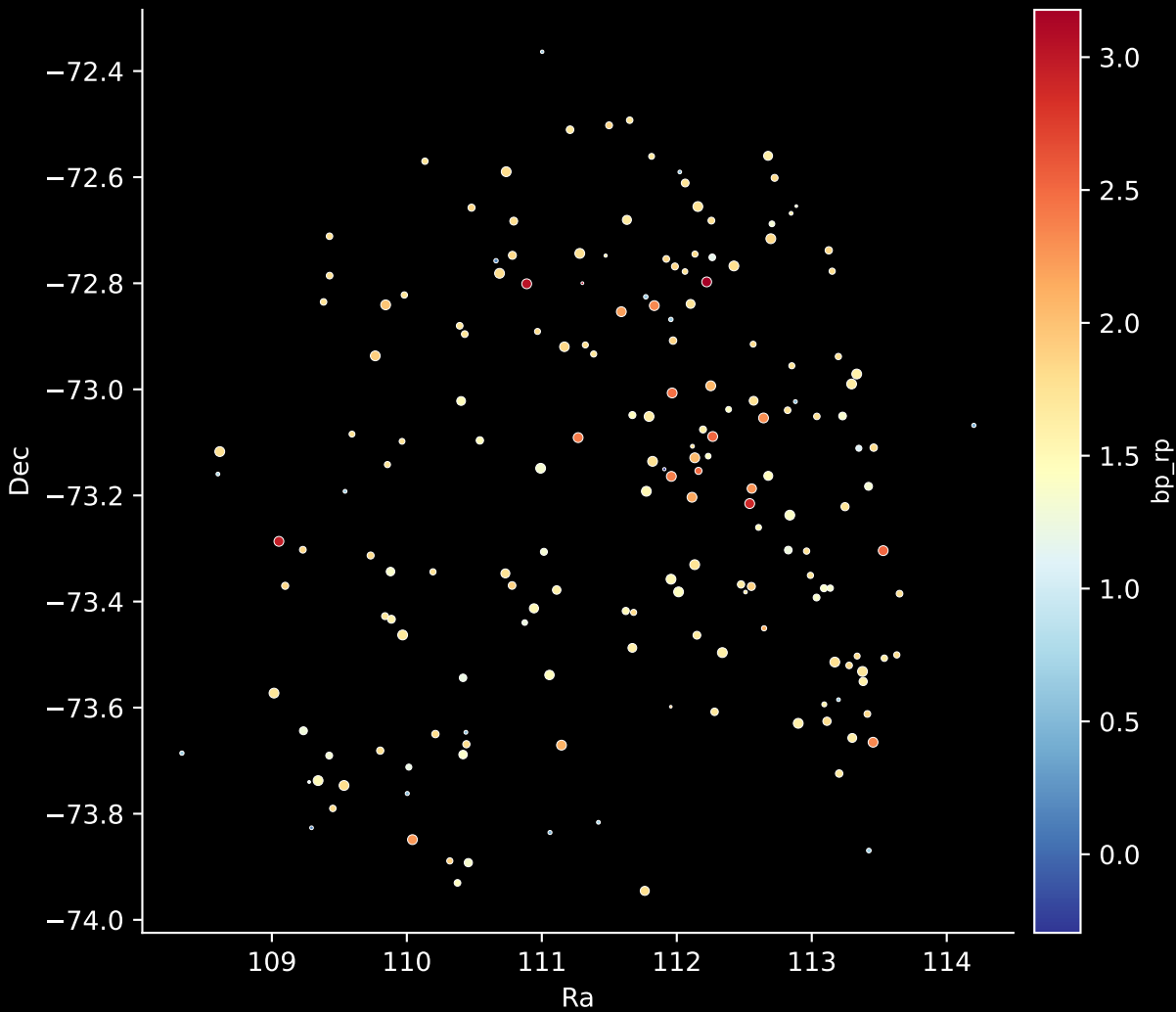
APOGEE DR17 Field: [SMC3] Stars: 180
