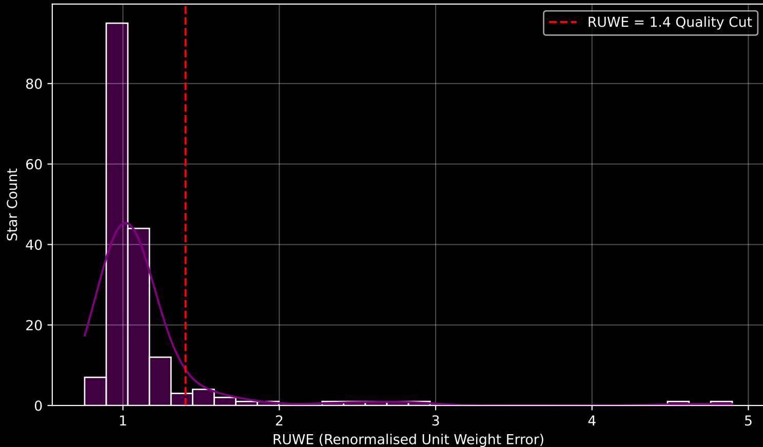
GAPOGEE DR17 Field [SMC3] RUWE Distribution (n= 176)
