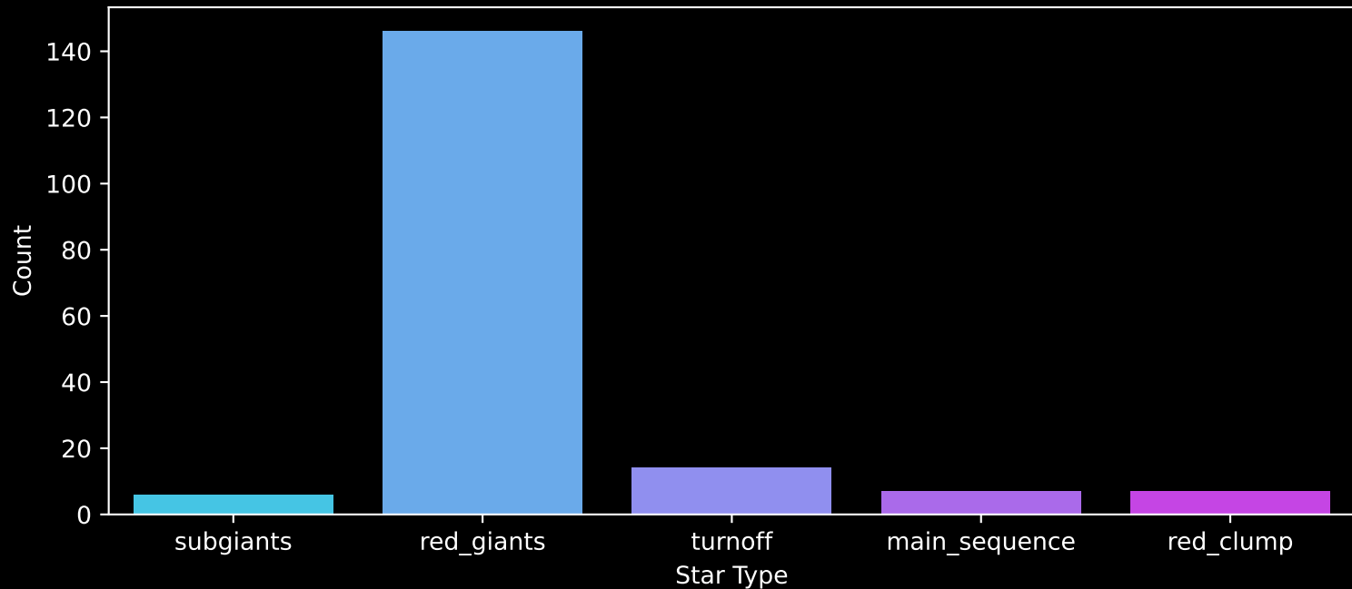
APOGEE DR17 Field: [SMC3] Count plot of Star Type
