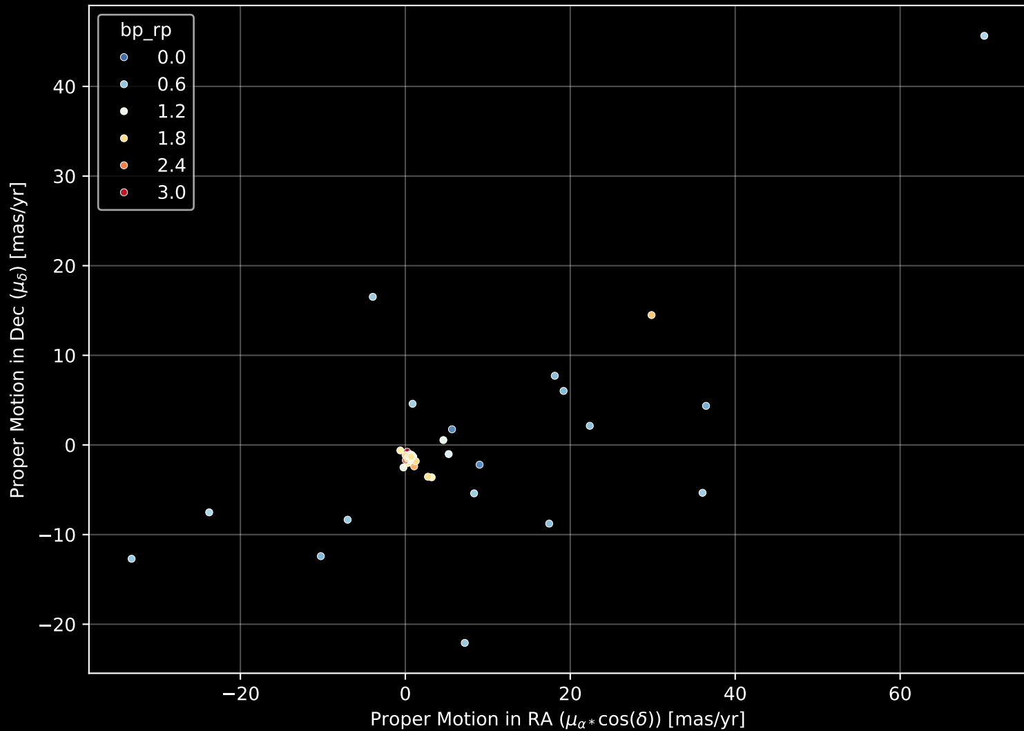
APOGEE DR17 Field: [SMC3] Proper Motion Diagram (n= 180)
