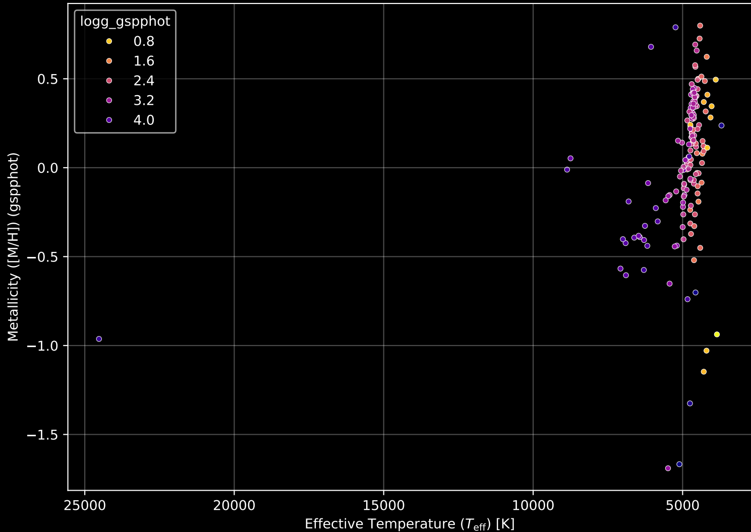
APOGEE DR17 Field: [SMC3] Stellar Population Parameters (n= 180)
